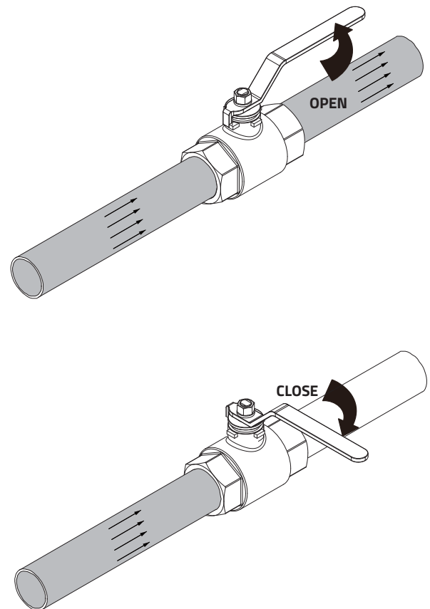
Figure 3.1 Rotation Direction for CLOSED and OPEN position
